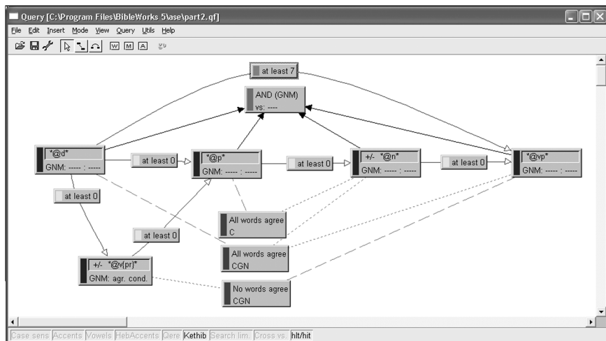
Figure 2. Example of a Graphical Search Interface
